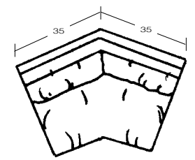
3335-50 ANGLED LOVESEAT H35 W57 D40 INSIDE: H17 W48 D25 SEAT H: 20 ARM H: 28
