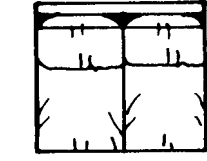
3335-46 ARMLESS LOVESEAT H35 W46 D40 INSIDE: H17 W46 D25 SEAT H: 20
