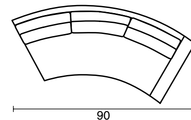
3909-1R RIGHT ARM WEDGE OUTSIDE: H33.5 W90 D37 INSIDE: H15.5 W68 D21 SEAT: H18.5 ARM: H25
