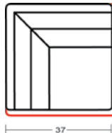
920-02-35 CORNER CHAIR 920-02-35/40 H36 W37 D37 INSIDE: H16 W22 D22 SEAT H: 20
