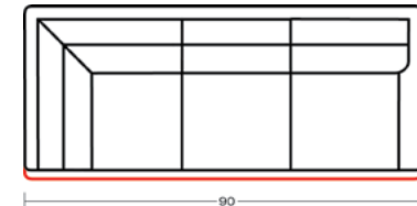
920-00R RIGHT ARM CORNER SOFA 920-00R/40 H36 W90 D37 INSIDE: H16 W74 D22 SEAT H: 20 ARM H: 24
