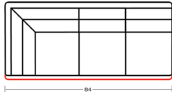
920-00-LC-10 LEFT CORNER ARMLESS SOFA 920-00-LC10/40 H36 W84 D37 INSIDE: H16 W72 D22 SEAT H: 20
