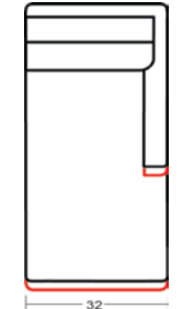
920-08-15 RIGHT ARM CHAISE 920-08-15/40 H36 W32 D62 INSIDE: H16 W26 D49 SEAT H:20 ARM H:24
